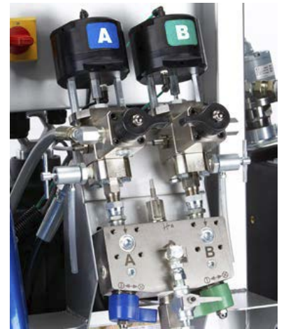
Standard blandingsmanifold
