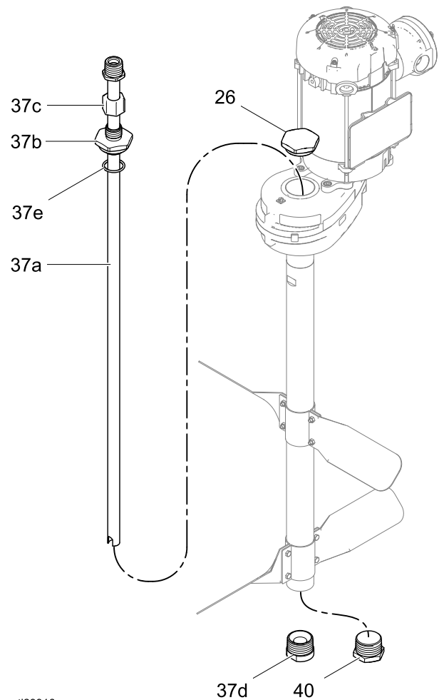
Figure 3 Siphon Tube
