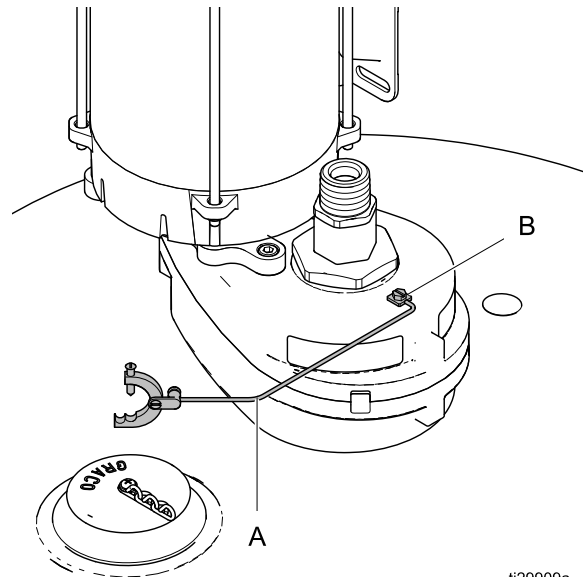
Figure 4 Agitator Ground
