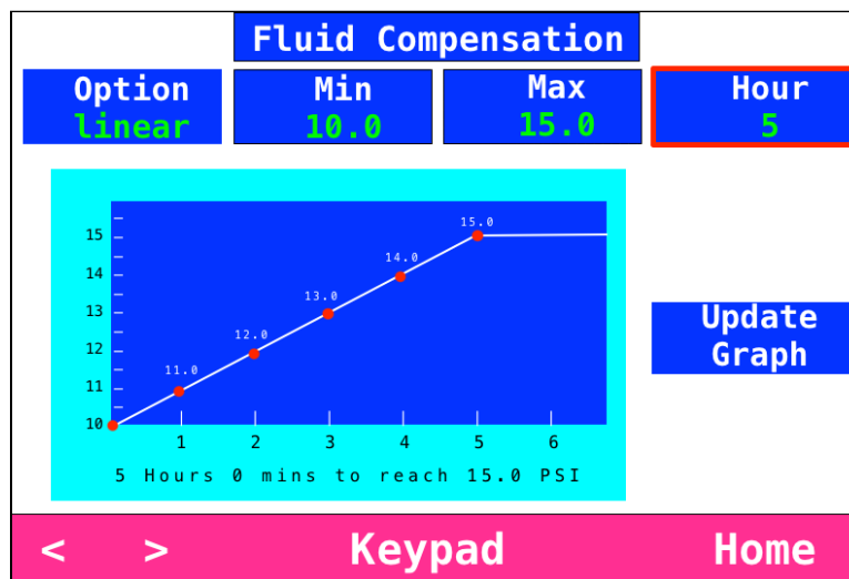
Figure 4-17: Pressure Curve for Sample Linear Program
