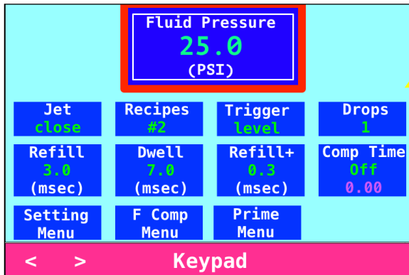
Figure 4-2: Touch Display Home Screen
