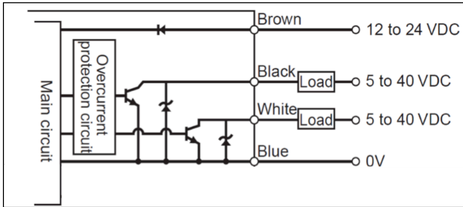
Schematic 5: Pressure Alarm Input/Output Circuit
