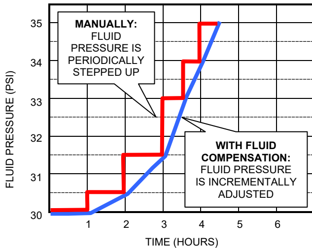
Figure 4-12: Fluid Pressure Adjusted Over Time
