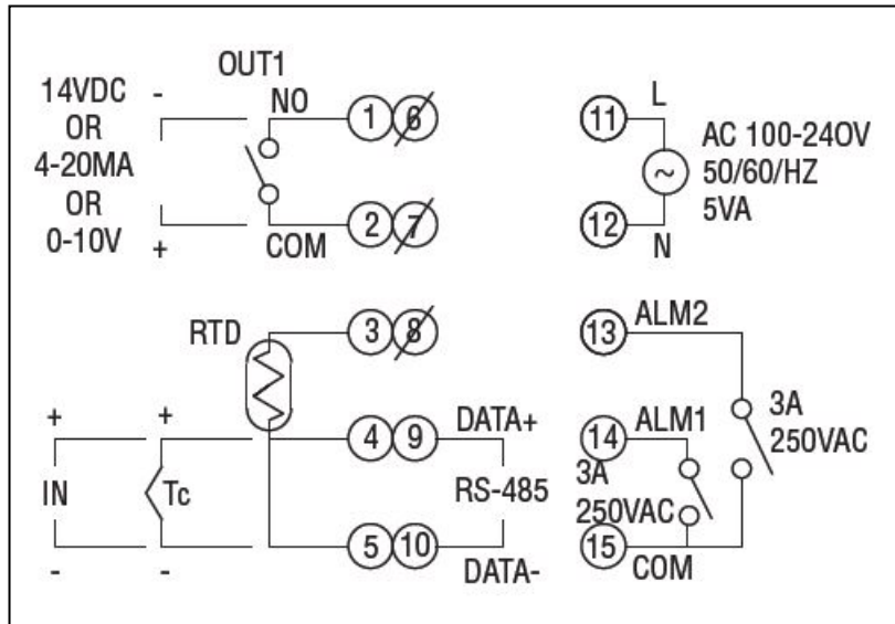
Schematic 4: Temperature Controller Connections
