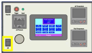
Figure 3-10: Jet and Fluid Pressure Regulators
