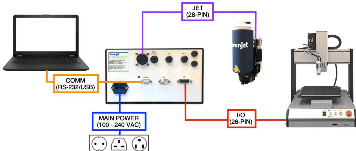
Figure 2-2: Cable Connections
