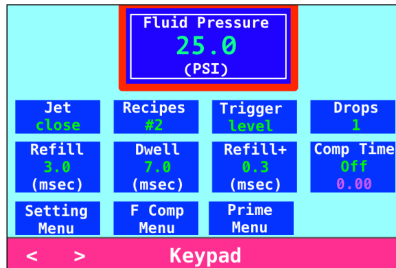
Figure 4-6: HM-2600C Home Screen
