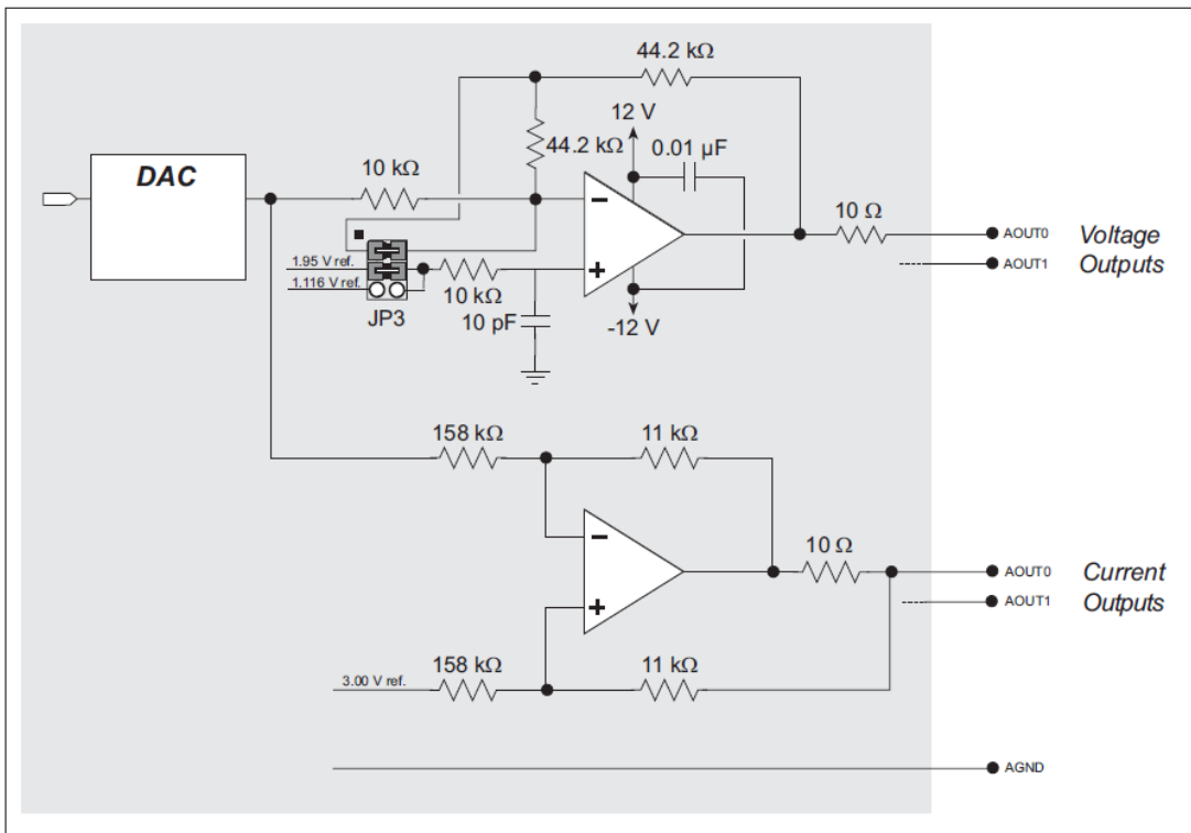
Schematic 3: D/A Converter Inputs
