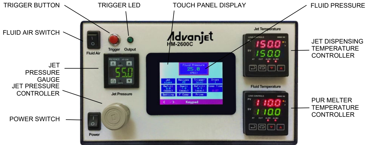
Figure 3-1: HM-2600C Front Panel
