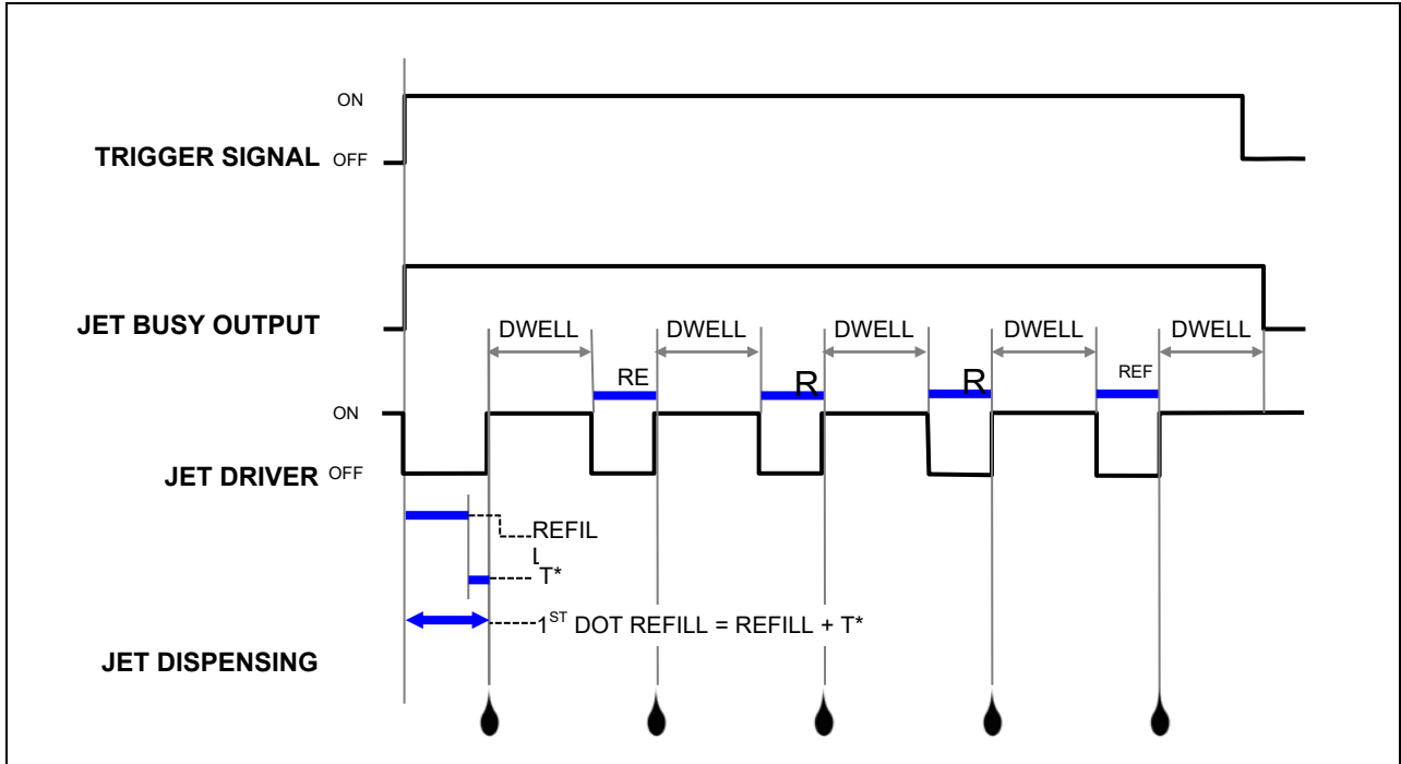
Figure A3- 2: 1 st Drop Compensation in LEVEL Mode, # of Drops = 1
