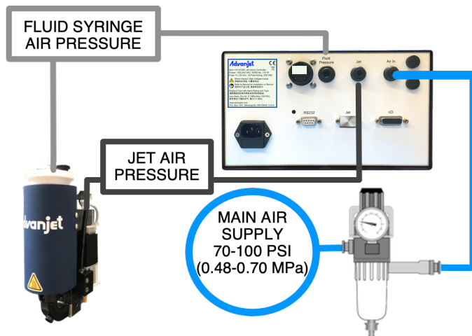
Figure 2-1: HM-2600C Pneumatic Connections
